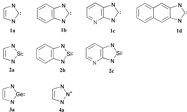
Scheme 2 Carbenes, silylenes, germylenes and nitrenium ions investigated (missing atoms are hydrogen).
