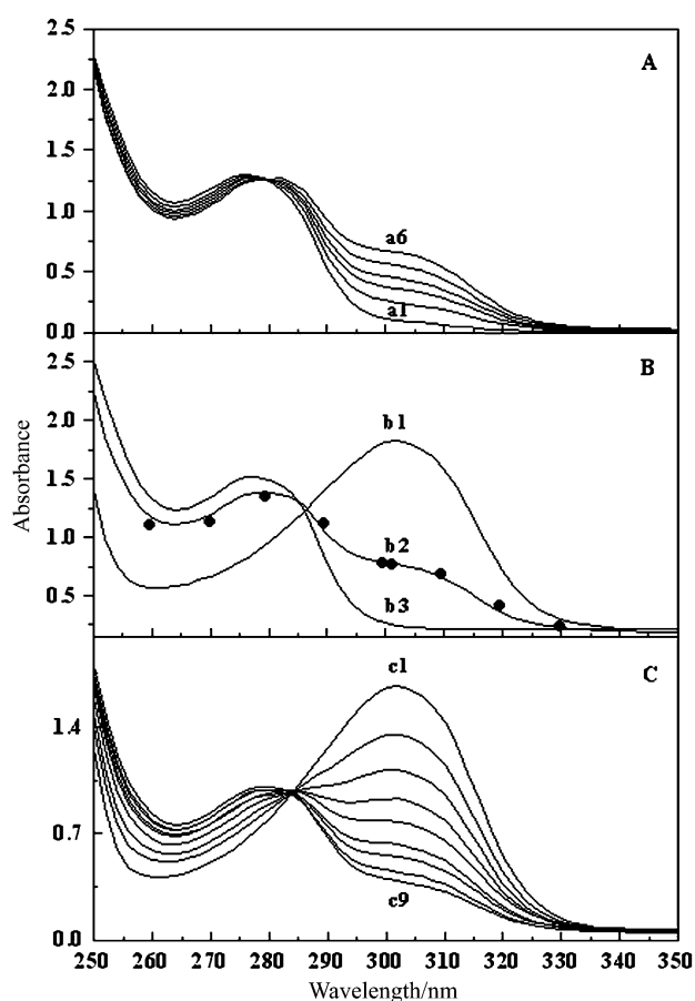
Fig. 1 Ultraviolet spectra in 5 M HCl, at 50 °C: Fig. 1A. Spectral variation obtained during the reaction of NCBL ( 1.0 \times 10^{-3} M). The time interval between each scan (a1–a6) is 3 min. Fig. 1B shows the spectra of (b1) N -phthaloylleucine ( 1.0 \times 10^{-3} M); (b2), solid line, refers to the observed spectra of the products of the NCBL reaction; the symbol (●) corresponds to the absorbance calculated for a solution composed of 6.67 \times 10^{-4} M phthalic acid and 3.33 \times 10^{-4} M N -phthaloylleucine; and (b3) corresponds to the spectra of phthalic acid ( 1.0 \times 10^{-3} M). Fig. 1C shows repetitive scans obtained during the reaction of N -phthaloylleucine, 1.0 \times 10^{-3} M. The time interval between each scan (c1–c9) is 24 hours.
