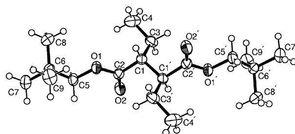
Fig. 2 ORTEP representation of meso -dineopentyl 2,3-diethylbutanedioate (50% probability ellipsoids).
