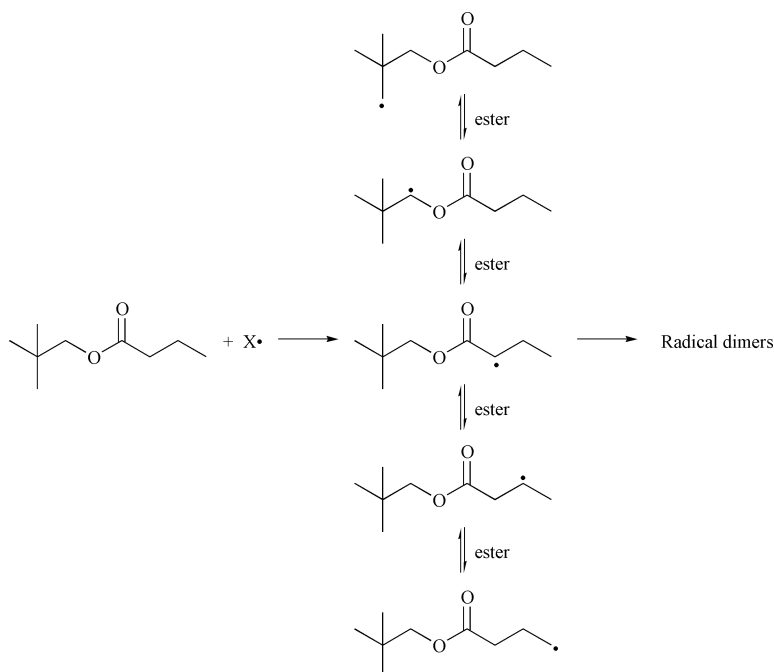
Scheme 4 Intermolecular rearrangement of ester radicals from neopentyl butanoate.
