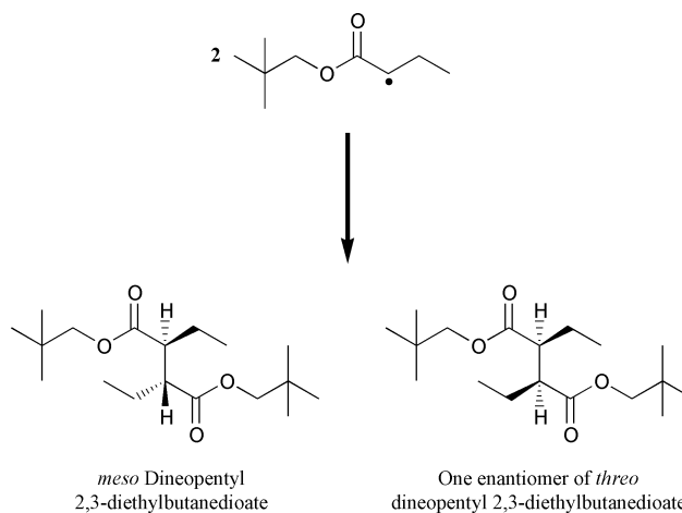
Scheme 2 The product diastereoisomers from the self-dimerisation of \alpha -acyl neopentyl butanoate radicals.
