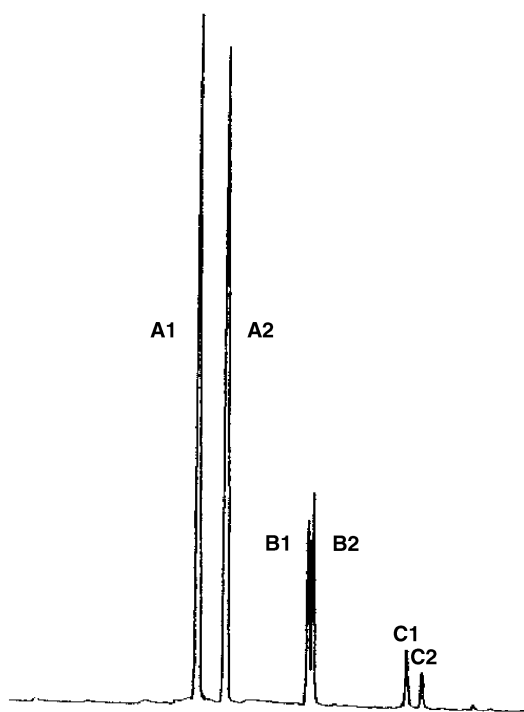
Fig. 1 GC chromatogram of the radical dimers formed by the thermolysis of DTBPO in neopentyl butanoate ( 1 ) at 438 K.
