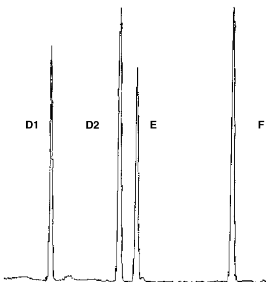
Fig. 4 GC chromatogram of the radical dimers formed by the thermolysis of DTBPO in neopentyl 2,2-dimethylpropanoate (2) at 438 K.
