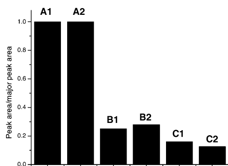
Fig. 6 The distribution of radical dimers from the thermolysis of neopentyl 2-bromobutanoate in neopentyl butanoate ( 1 ) at 438 K.
