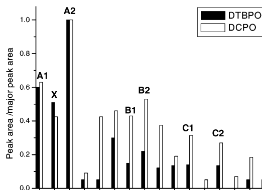
Fig. 5 The distribution of radical dimers from the photolysis of DTBPO and DCPO in neopentyl butanoate (1) at 298 K.
