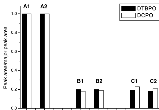
Fig. 3 The distribution of radical dimers from the thermolysis of DTBPO and DCPO in neopentyl butanoate (1) at 438 K.
