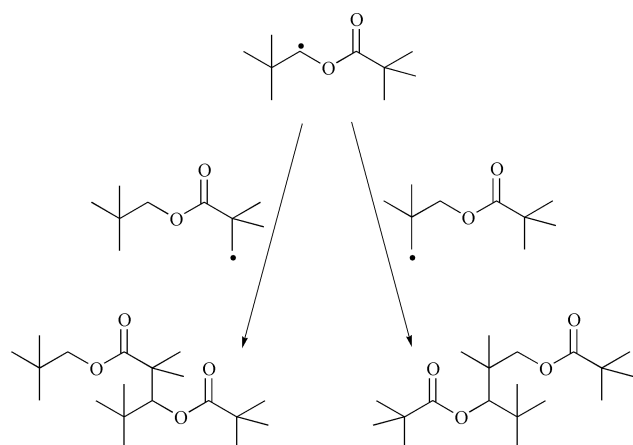
Scheme 3 Cross-dimerisation of \alpha -alkyl and primary radicals of neopentyl 2,2-dimethylpropanoate.
