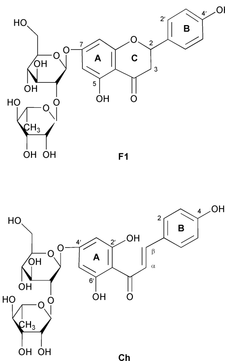
Scheme 1 Chemical structure of naringin, Fl (7-rhamnoglucosyl-4',5-dihydroxyflavanone) and its chalcone, Ch (4'-rhamnoglucosyl-2',6',4-trihydroxychalcone).
