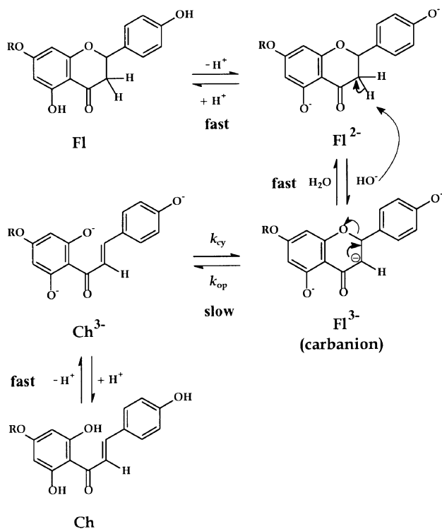
Scheme 2 Carbanion intermediate mechanism for the flavanone–chalcone isomerisation equilibrium of naringin in basic media.
