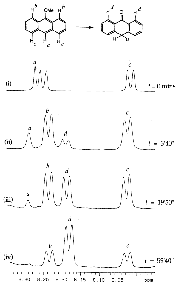
Fig. 4 Proton NMR spectra (500 MHz) of 9-methoxyanthracene in DCl– \text{D}_2\text{O} – \text{CD}_3\text{CN} (~6.7 M) showing extents of exchange and hydrolysis at different time intervals.
