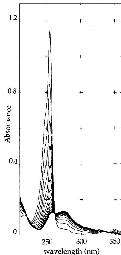
Fig. 1 Repetitive scans of UV spectra for hydrolysis of 9-methoxyanthracene to anthrone ( 1.2 \times 10^{-5} \text{ M} substrate in 4.9 M \text{HClO}_4 ).
