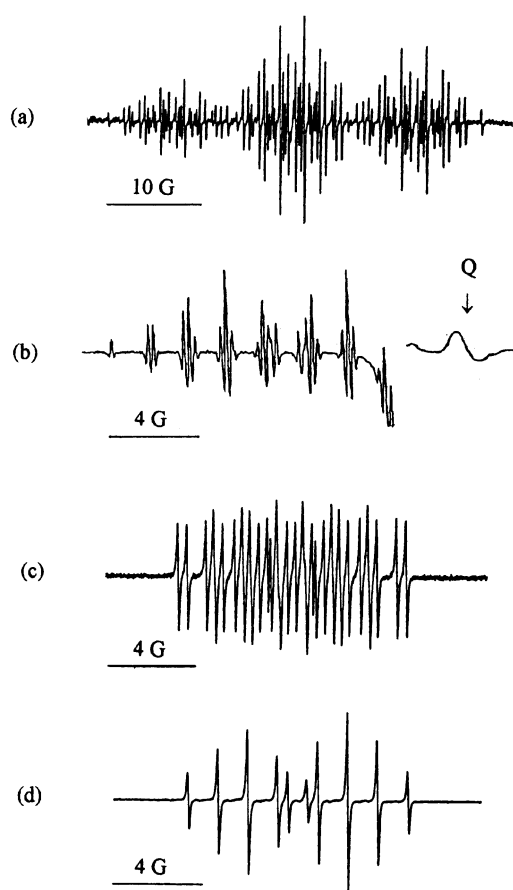
Fig. 1 (a) EPR spectrum obtained upon photolysis of 2-hydroxypyrimidine in the presence of triethylamine (radical 1 ); (b) EPR spectrum obtained on electron irradiation of 4,5,6-trihydroxypyrimidine in the presence of sodium formate (radical 3 ). Q denotes the quartz signal; (c) EPR spectrum obtained upon photolysis of 4,5,6-trihydroxypyrimidine with potassium persulfate at pH = 8.3 (radical 14 ); and (d) pH = 12.1 (radical 15 ).
