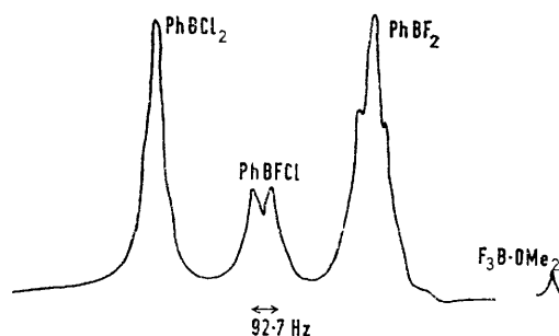
32.1 MHz ^{11}\text{B} N.m.r. spectrum of a mixture of \text{PhBF}_2 and \text{PhBCl}_2 in methylcyclohexane at 303 K
