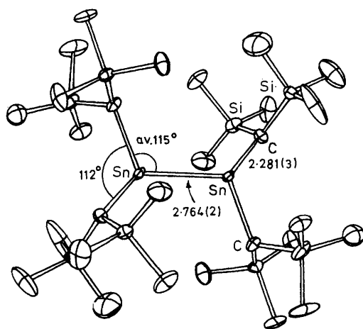
Crystal and molecular structure of \text{Sn}[\text{CH}(\text{SiMe}_3)_2]_2
