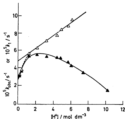
Dependences of k_{obs} (▲) and k_1 (△) on [H + ] at 80 °C
