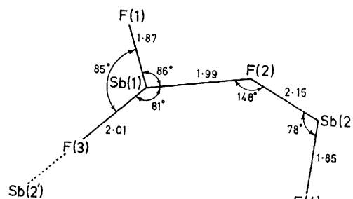
FIGURE 2 The [\text{Sb}_2\text{F}_4]^{2+} cation. Bond lengths in \text{\AA}
