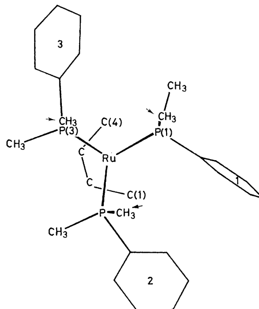
FIGURE 2 Projection of the molecule on to the plane of the three phosphorus atoms. Arrows indicate the three methyl groups which are forced together and for which the Ru-P-C(methyl) angle is 122^\circ
