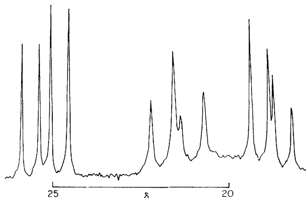
FIGURE 2 ^{31}\text{P}\{-^1\text{H}\} n.m.r. spectrum (36.4 MHz) of (9) \text{N}_3\text{P}_3(\text{NHCH}_2\text{CH}_2\text{NH})\text{Ph}_2\text{Cl}_2
