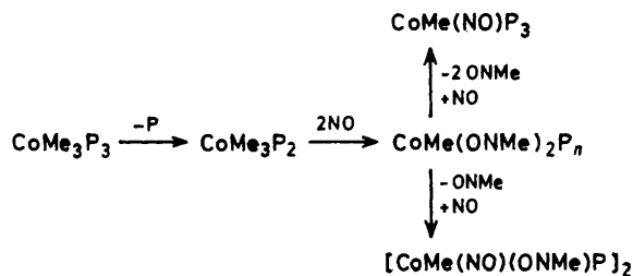
SCHEME 1 P can be \text{PMe}_3 and/or \text{POMe}_3
