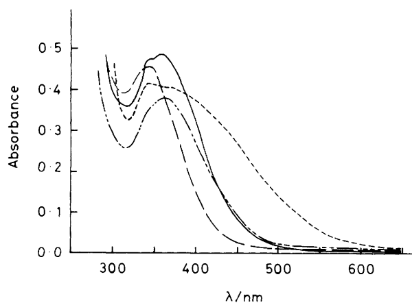
Figure 1. Charge-transfer spectra of 1.0 \times 10^{-4} mol dm -3 solutions of [CeCl 4 (dmsso) 3 ] (—), [CeCl 4 (apn) 2 ] (---), [CeCl 4 (tpao) 2 ] (- - -), and [CeCl 4 (dmdap) 2 ] (----) in methylene dichloride
