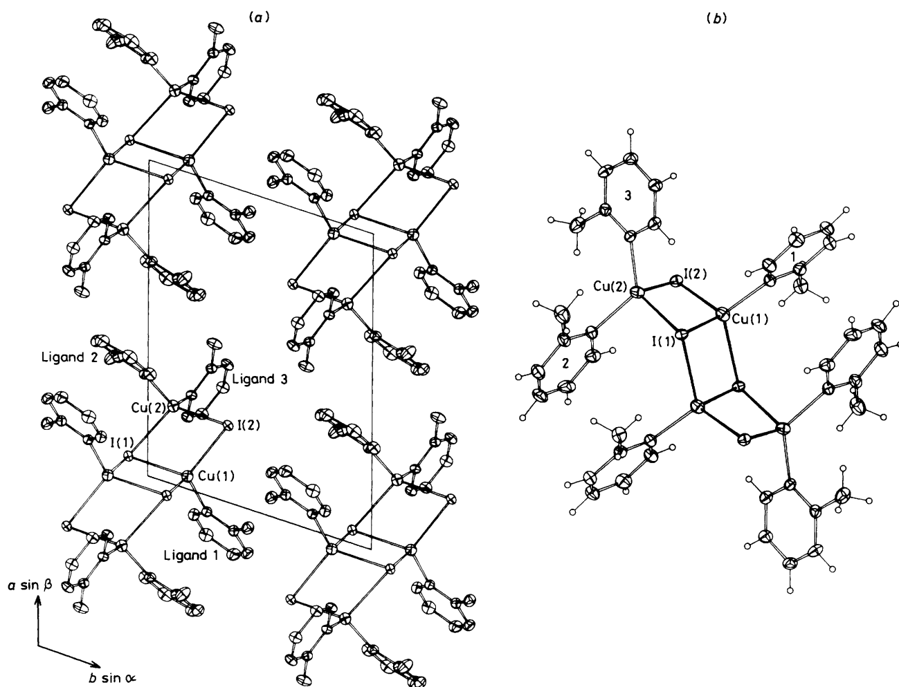
Figure 5. (a) Unit-cell contents of complex (5) projected down c ; 20% thermal ellipsoids are shown for the non-hydrogen atoms. (b) Projection of a single molecule of (5)
