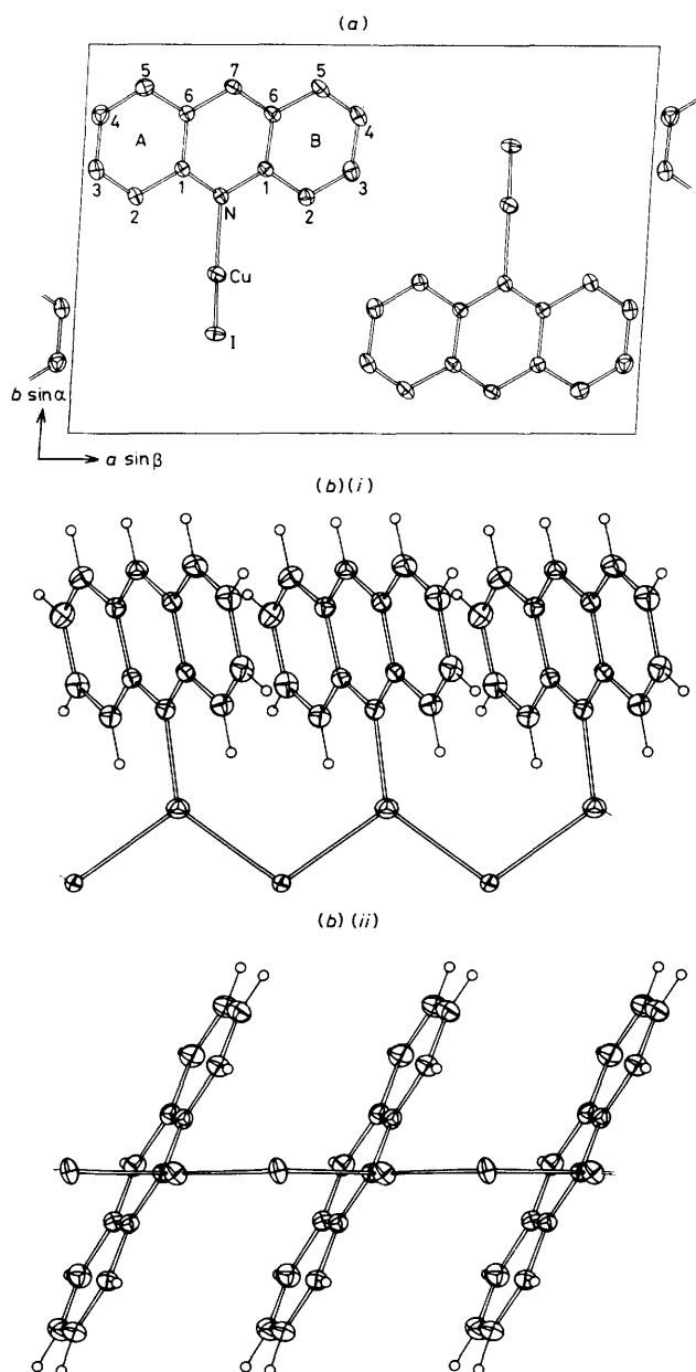
Figure 4. (a) Unit-cell contents of complex (4) projected down c . (b) A projection of the polymer of (4), (i) normal to the (CuI)_{\infty} plane, (ii) through the bisector of I-Cu-I
