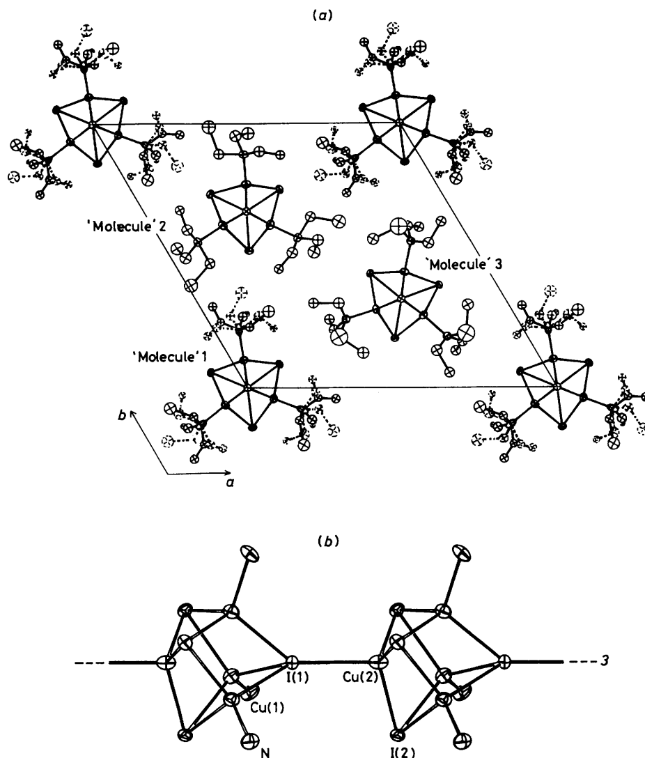
Figure 1. (a) Unit-cell contents of complex (1) projected down c ; 20% thermal ellipsoids are shown for the non-hydrogen atoms. (In the case of carbon atoms these are spheres.) (b) A segment of polymeric string 3 in (1). In all polymer strings, I(1) and Cu(2) are axial and bonded to each other, thus lying in successive cubes. Cu(1) and I(2) are off-axis and are bonded to and lie in the same cubes as I(1) and Cu(2) respectively
