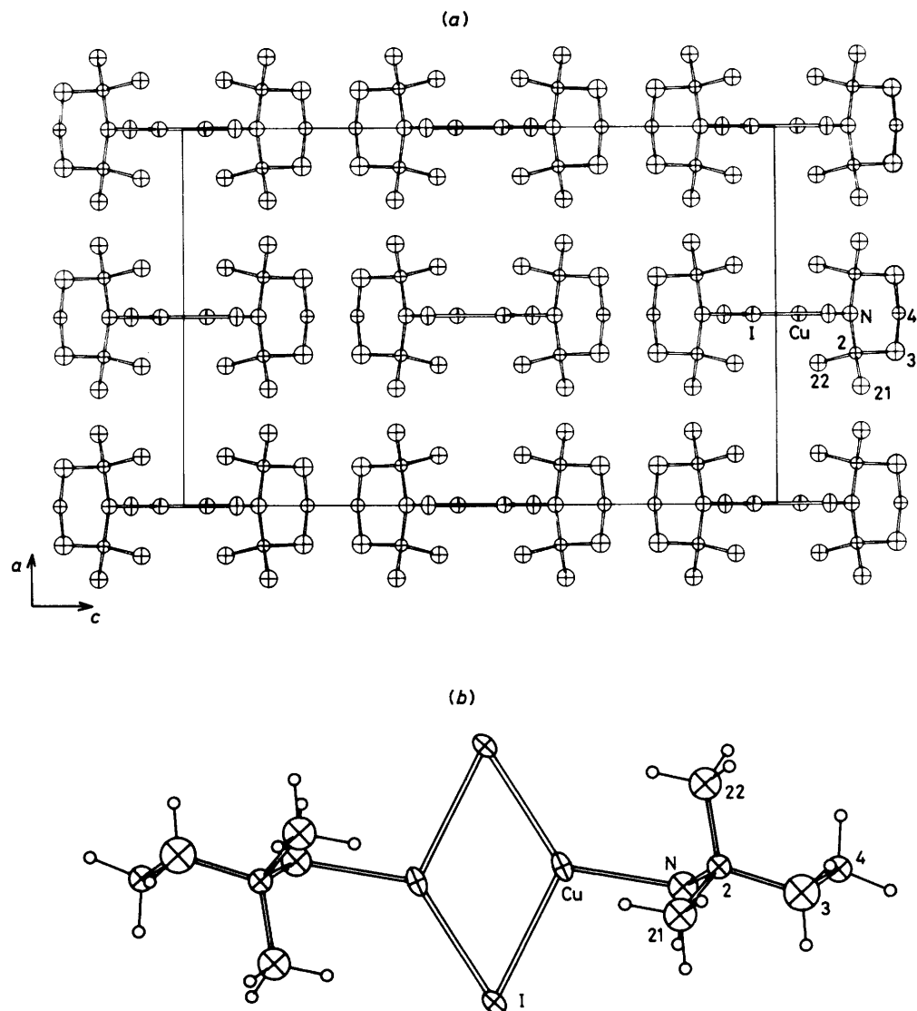
Figure 3. (a) Unit-cell contents of complex (3) projected down b . (b) A projection of the dimer of (3) normal to the \text{Cu}_2\text{I}_2 ring plane
