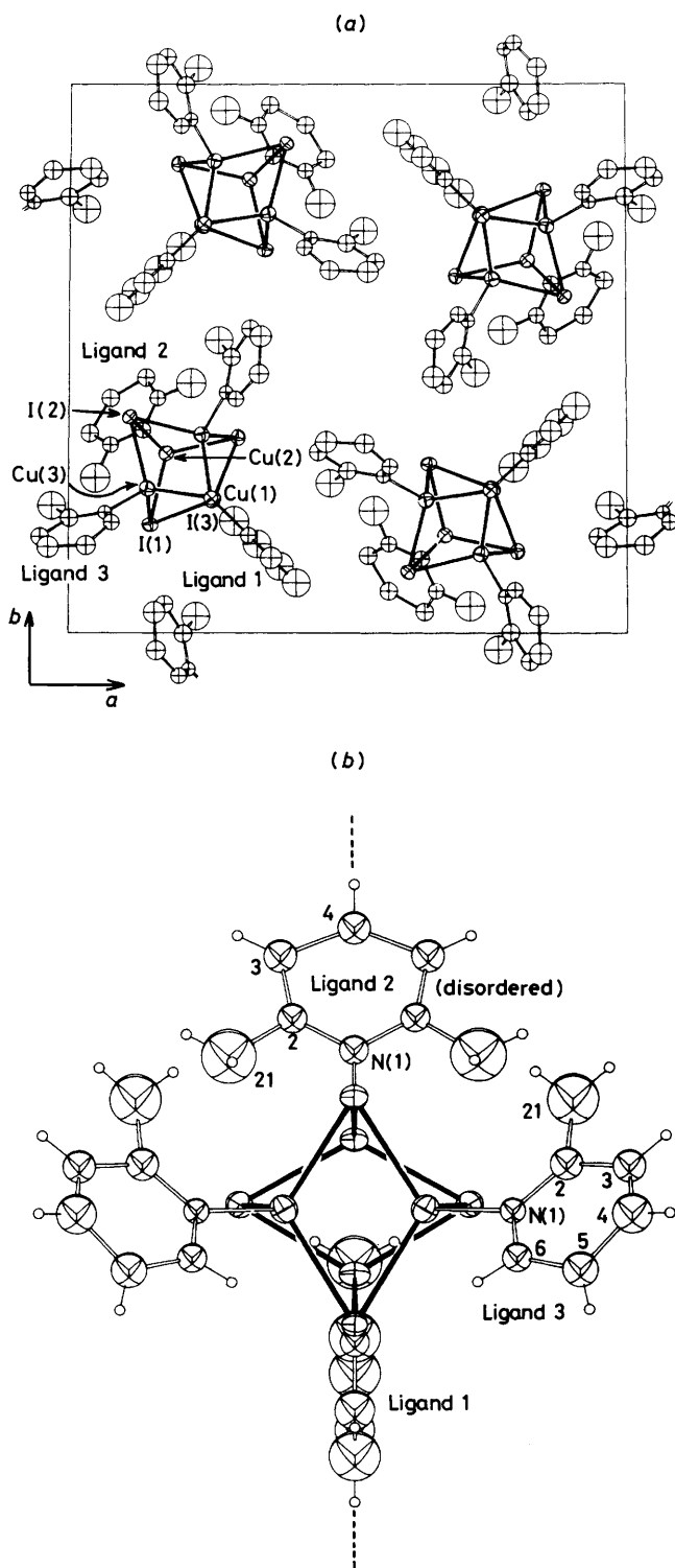
Figure 2. (a) Unit-cell contents of complex (2) projected down c ; 20% thermal ellipsoids are shown for the non-hydrogen atoms, only those for Cu and I being anisotropic. (b) A projection of the molecule of (2) showing the ligand numbering
