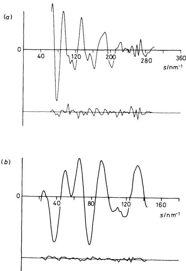
Figure 3. Experimental and final-difference molecular-scattering intensities for \text{Me}_3\text{N}\cdot\text{GaH}_3 ; nozzle-to-plate distances (a) 128.3 and (b) 285.7 mm
