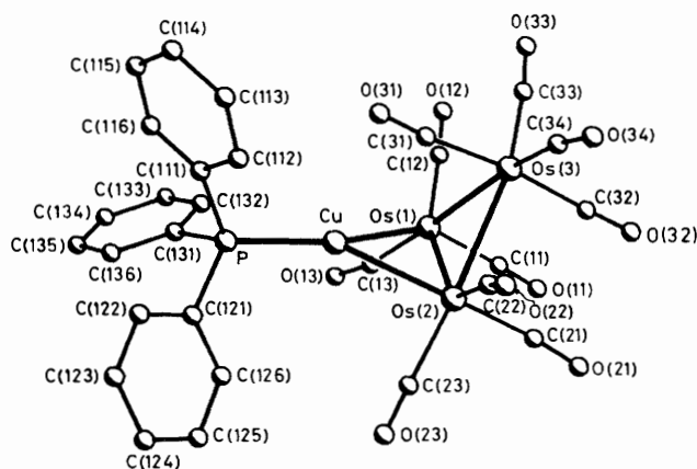
Figure 1. The molecular structure of [\text{Os}_3\text{H}_3(\text{CO})_{10}\{\text{Cu}(\text{PPh}_3)\}] (1) including the atom numbering scheme adopted; hydrogen atoms have been omitted for clarity
