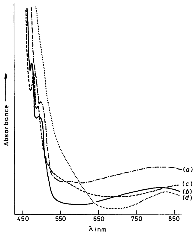
Figure 2. Absorption spectra of \text{Na}[\text{Fe}^{\text{III}}(\text{edta})] in dmf (a), dmsO (b), \text{H}_2\text{O} (c), and methanol (d)
