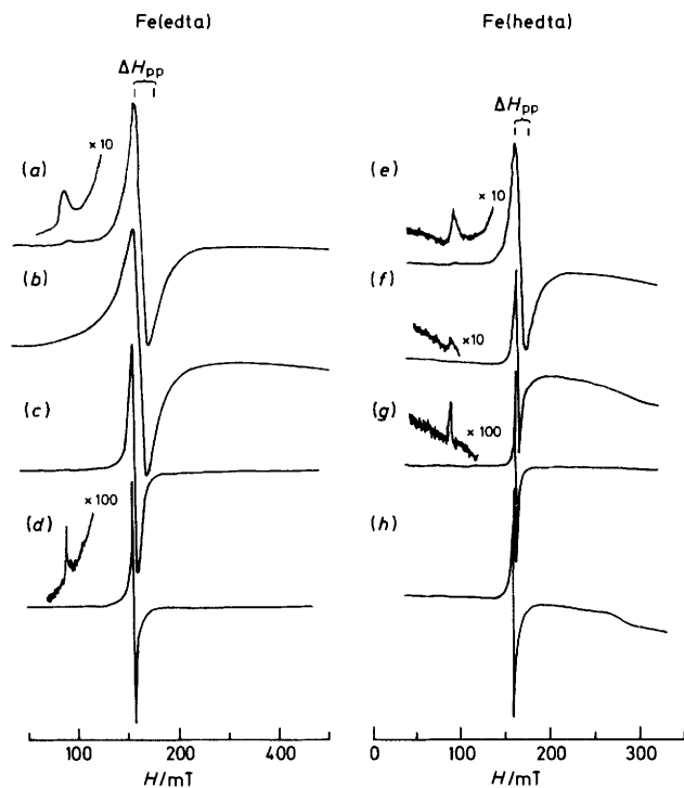
Figure 1. E.s.r. spectra obtained from \text{Na}[\text{Fe}^{\text{III}}(\text{edta})] (1 mmol \text{dm}^{-3} ) in \text{H}_2\text{O} (pH 7) (a), dmsO (b), dmf (c), methanol (d) and from \text{Fe}^{\text{III}}(\text{hedta}) in \text{H}_2\text{O} (pH 7) (e), methanol (f), dmf (g), dmsO (h). Recorded at 77 K
