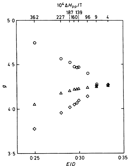
Figure 3. Plot of high-spin iron(III) g values [ (\Delta) g_x, (\diamond) g_y, (O) g_z ] for the middle Kramers doublet as a function of the rhombicity of the field ( E/D ) and the peak-to-peak linewidth, \Delta H_{pp} , estimated from the difference of the resonant field corresponding to the largest and the smallest principal g values. D = 0.74 \text{ cm}^{-1} , B = 0.16 \text{ T}
