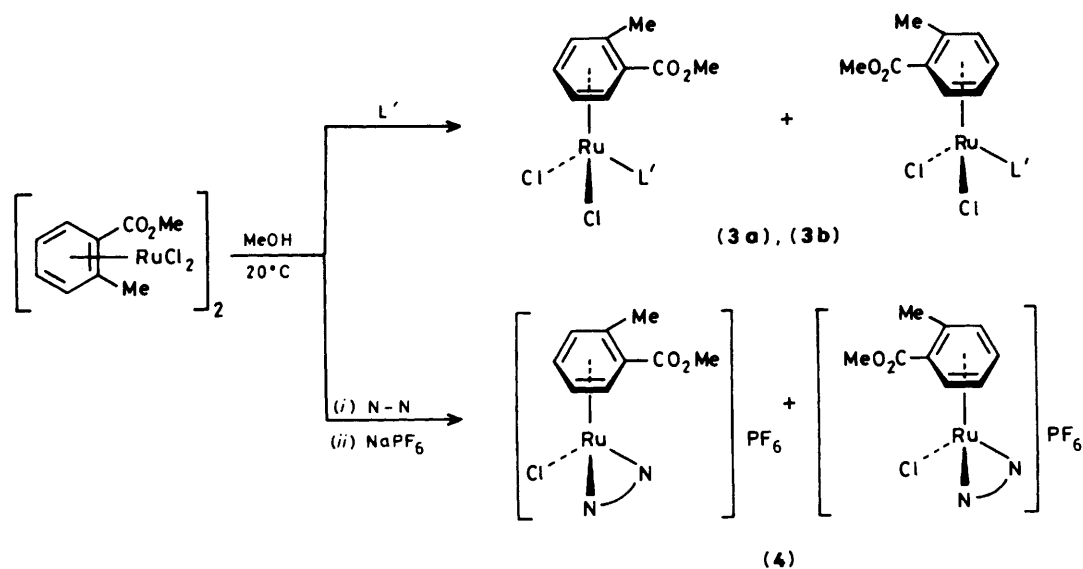
Scheme 2. L' = (-)(S)-1-Phenylethylamine, (3a); or (+)-dehydroabietylamine, (3b). N-N = (-)(R,R)-1,2-diphenyl-1,2-diaminoethane. (4)
