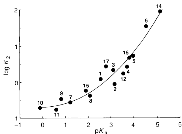
Fig. 2 Dependence of the stability of the [\text{AuCl}_3(\text{L})] complexes upon ligand basicity (L is identified by its number in Table 4)
