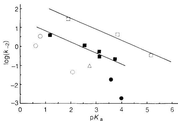
Fig. 3 Plots of \log k_{-2} versus pK_a for ( \square ) pyridines, ( \blacksquare ) unhindered thiazoles and those with a single ortho -methyl substituent, ( \circ ) oxazole, 2-methylbenzoxazole and 2-methylbenzothiazole, ( \bullet ) 2,4-dimethylthiazole and 2,4,5-trimethyloxazole and ( \triangle ) 2,6-bis(chloromethyl)pyridine
