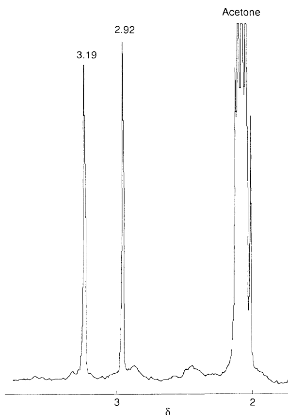
Fig. 1 Proton NMR spectrum of trichloro(2,5-dimethyl-1,3,4-thiadiazole)gold(III)
