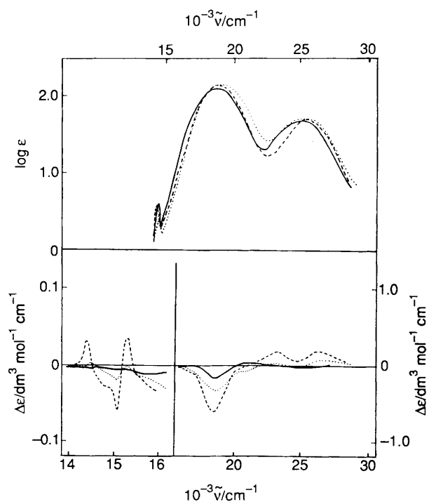
Fig. 1 Absorption (upper) and CD (lower) spectra for three diastereoisomers of [\text{Cr}\{(S)\text{-pdtp}\}]^- in \text{H}_2\text{O} : P-I (—), P-II (⋯), and P-III (---)
