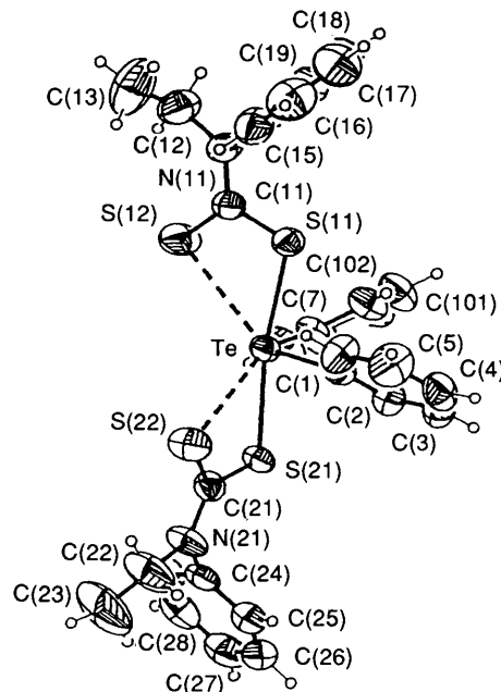
Fig. 7 View of \text{Ph}_2\text{Te}(\text{S}_2\text{CNETPh})_2 6 , showing the atomic numbering
