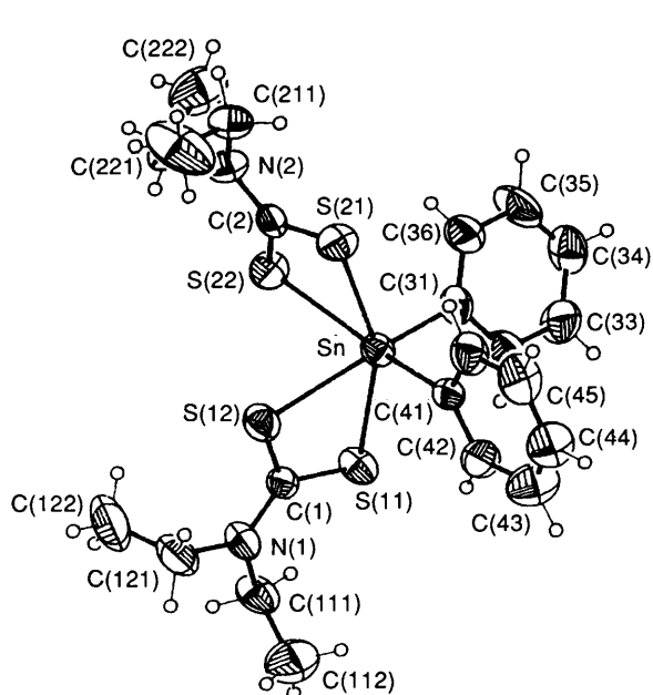
Fig. 5 View of \text{Ph}_2\text{Sn}(\text{S}_2\text{CNET}_2)_2 3 , showing the atomic numbering
