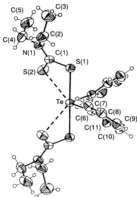
Fig. 6 View of \text{Ph}_2\text{Te}(\text{S}_2\text{CNET}_2)_2 5 , showing the atomic numbering
