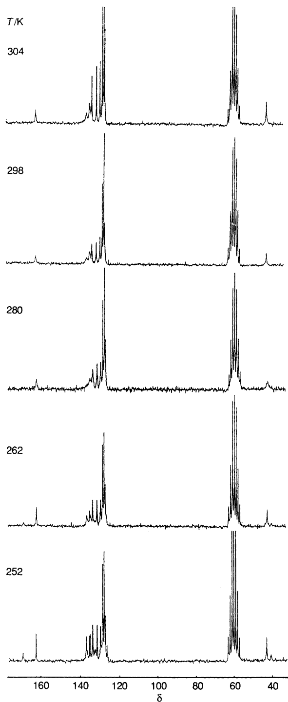
Fig. 3 Variable-temperature ^{13}\text{C}\{-^1\text{H}\} NMR spectra of [\text{CuL}]\text{ClO}_4 in \text{CD}_3\text{NO}_2 showing the equilibrium between [(\pm)\text{-}(R^*,R^*,R^*)] and [(\pm)\text{-}(R^*,S^*,S^*)] diastereomers
