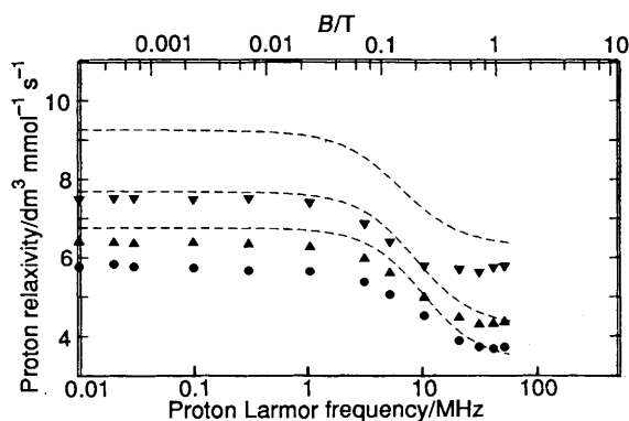
Fig. 4 The 1/T_1 NMRD profiles for an aqueous solution of [GdL], as a function of temperature ( \nabla , 5; \blacktriangle , 25; \bullet , 35 °C), expressed in relaxivity units (the rate increase per mmol dm -3 of added paramagnetic ion). The dashed curves are the data for [Gd(dtpa)] 2- at the same temperatures
