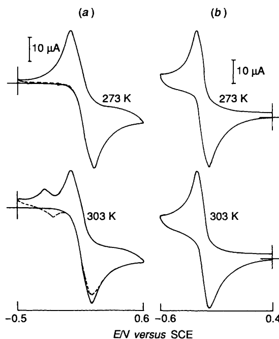
Fig. 7 Variable-temperature cyclic voltammograms (scan rate 50 \text{ mV s}^{-1} ) of \approx 10^{-3} \text{ mol dm}^{-3} solutions of (a) cis - [\text{OsL}_2(\text{PPh}_3)_2][\text{PF}_6] [first cycle (—), second cycle (---)] and (b) trans - [\text{OsL}_2(\text{PPh}_3)_2]\text{PF}_6 in dichloromethane
