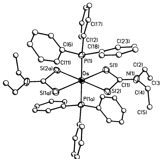
Fig. 3 Perspective view and atom labelling scheme for trans - [\text{OsL}_2(\text{PPh}_3)_2]
