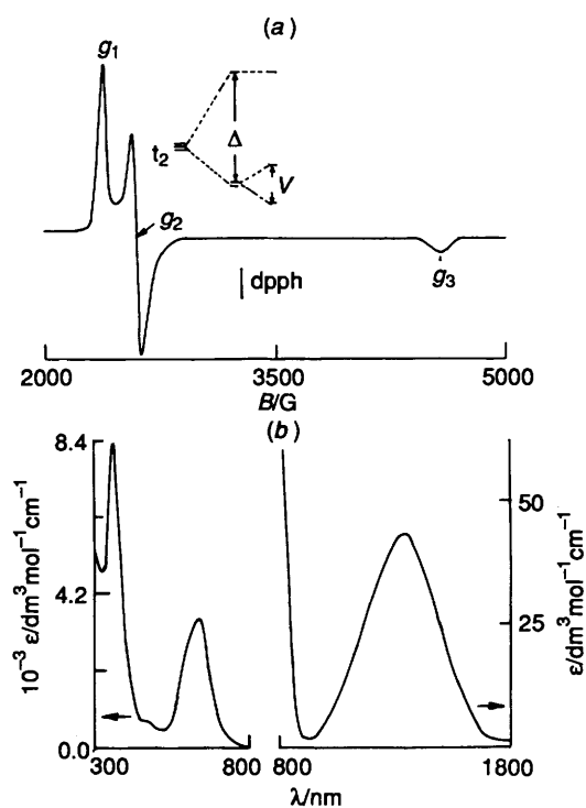
Fig. 1 (a) X-Band EPR spectrum and t_2 splittings of trans - [\text{OsL}_2(\text{PPh}_3)_2]\text{PF}_6 in dichloromethane-toluene (1:1) glass (77 K): g_1 = 2.7645 , g_2 = 2.5249 , g_3 = 1.4368 , \Delta = 7530 \text{ cm}^{-1} , V = 1930 \text{ cm}^{-1} , G = 10^{-4} \text{ T} . (b) Electronic spectrum of trans - [\text{OsL}_2(\text{PPh}_3)_2]\text{PF}_6 in dichloromethane at 298 K
