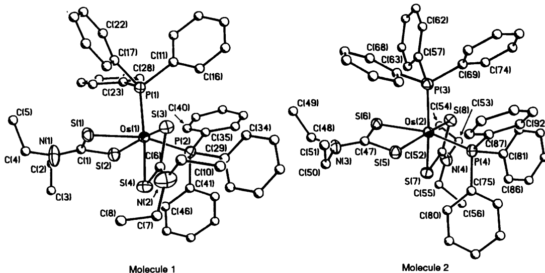
Fig. 2 Perspective view and atom labelling scheme for the two independent molecules of cis - [\text{OsL}_2(\text{PPh}_3)_2]
