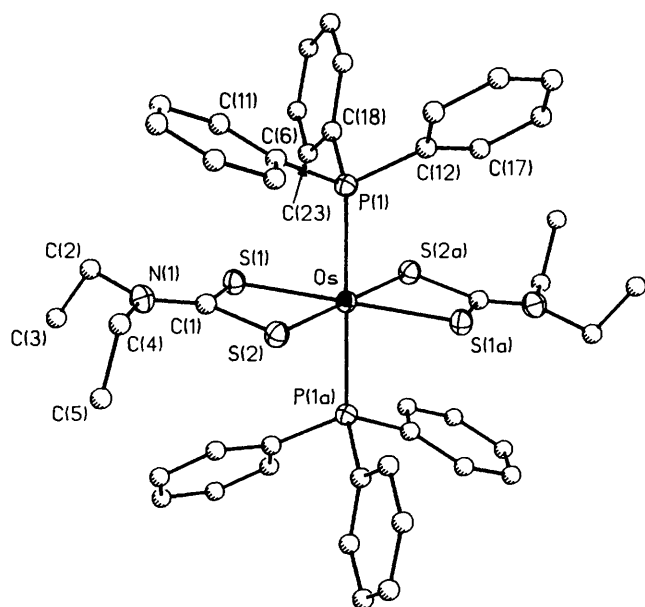
Fig. 4 Perspective view and atom labelling scheme for the cation of trans -[OsL 2 (PPh 3 ) 2 ] + PF 6 -
