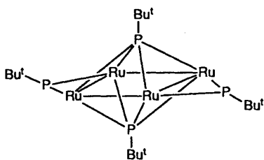
Fig. 2 Schematic representation of the molecular structure of [\text{Ru}_4(\text{CO})_8(\text{P}^t\text{Bu})_4] 2
