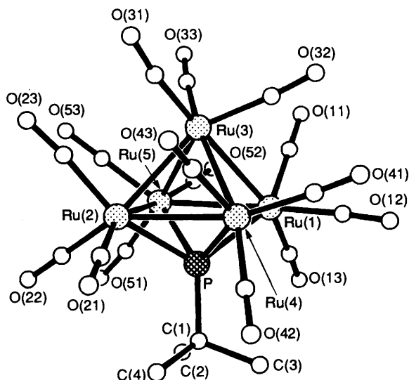
Fig. 3 The molecular structure of [\text{Ru}_5(\text{CO})_{15}(\text{P}^t\text{Bu})] 3
