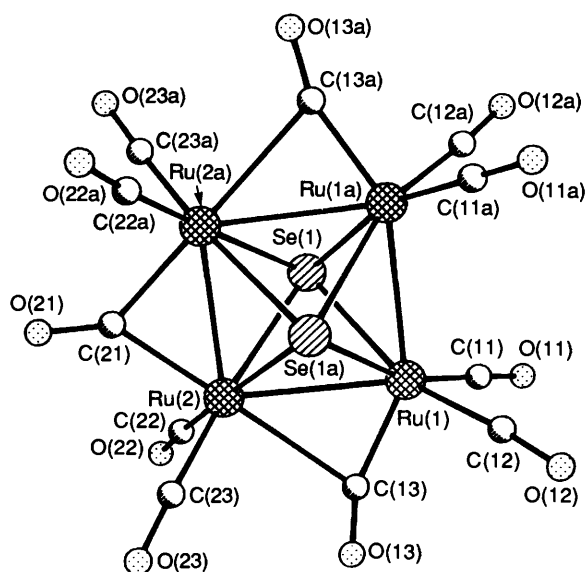
Fig. 6 The molecular structure of [\text{Ru}_4(\mu_4\text{-Se})_2(\text{CO})_8(\mu\text{-CO})_3] \mathbf{5}
