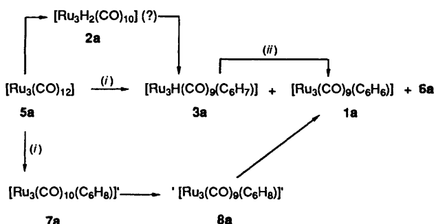
Scheme 3 Formation of [\text{Ru}_3(\text{CO})_9(\text{C}_6\text{H}_6)] from [\text{Ru}_3(\text{CO})_{12}] : (i) reaction with \text{Me}_3\text{NO}\cdot\text{CH}_2\text{Cl}_2 in the presence of 1,3- \text{C}_6\text{H}_8 ; (ii) heating in hexane
