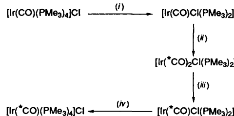
Scheme 2 (i) Sublimation, -2 \text{PMe}_3 ; (ii) ^{13}\text{C} , hexane; (iii) vacuum, -\text{CO} ; (iv) +2 \text{PMe}_3 , benzene. * Indicates approximately 50% ^{13}\text{C} enrichment
