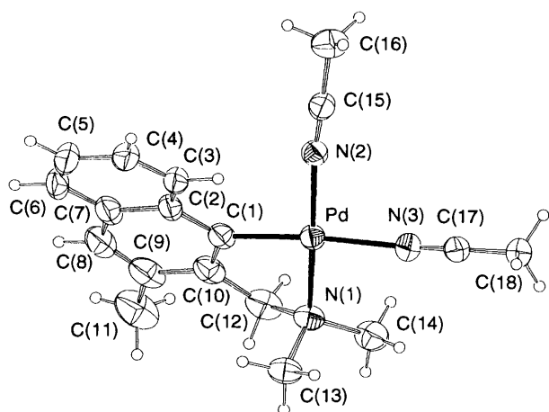
Fig. 1 An ORTEP 15 drawing (30% probability level) of the molecular structure of complex 7a together with the numbering scheme adopted (the CF 3 SO 3 - fragment is omitted for clarity)
