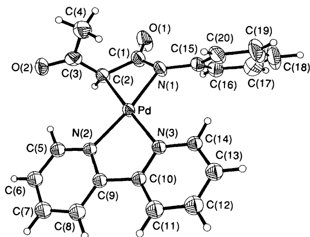
Fig. 1 Molecular structure of [\text{Pd}\{\text{CH}(\text{COMe})\text{C}(\text{O})\text{NPh}\}(\text{bipy})] 2a showing the atom numbering scheme. Atoms are shown as thermal ellipsoids at the 50% probability level
