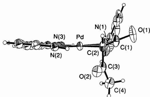
Fig. 2 Side view of [\text{Pd}\{\text{CH}(\text{COMe})\text{C}(\text{O})\text{NPh}\}(\text{bipy})] 2a , showing the puckering of the palladalactam ring
