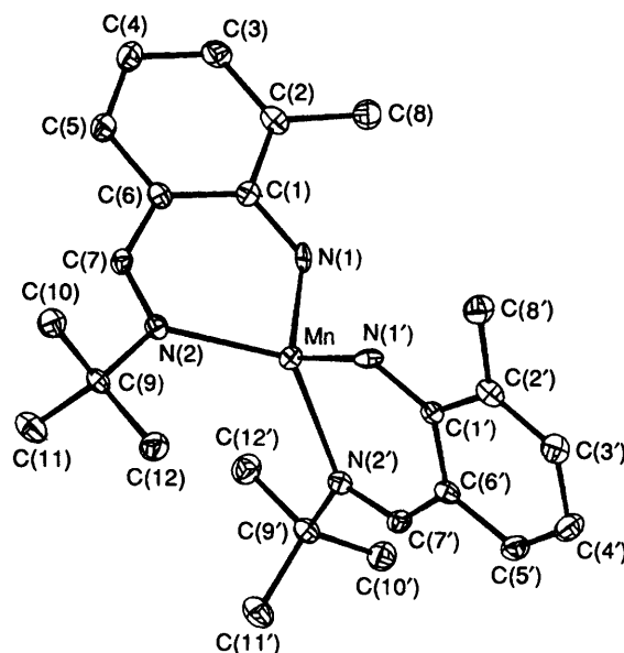
Fig. 2 Structure of \text{Mn}[\text{N}(\text{Bu}')=\text{C}(\text{H})\text{C}_6\text{H}_3(\text{Me})\text{NH}]_2 4
