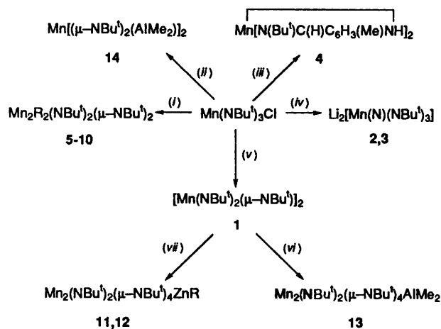
Scheme 1 Main reactions of \text{Mn}(\text{NBu}^t)_3\text{Cl} . (i) \text{LiMe} , dme; \text{ZnR}_2 , thf, \text{R} = \text{Me} , Et, \text{CH}_2\text{Bu}^t , \text{CH}_2\text{CMe}_2\text{Ph} , \text{CH}_2\text{SiMe}_3 , \text{CH}_2\text{Ph} ; (ii) \text{Li}(\text{NHBu}^t) , dme, to give [\text{Li}(\text{dme})]_2[\text{Mn}(\text{NBu}^t)_4] (ref. 1), then \text{Al}_2\text{Me}_6 in light petroleum; (iii) excess \text{Li}(\text{NHC}_6\text{H}_3\text{Me}_2\text{-2,6}) , dme; (iv) excess \text{Li}(\text{NHBu}^t) , dme–light petroleum or thf; (v) \text{Li}(\text{NHBu}^t) , \text{Et}_2\text{O} , then \text{O}_2 ; (vi) \text{Al}_2\text{Me}_6 toluene; (vii) \text{ZnR}_2 , \text{R} = \text{Me} , \text{CH}_2\text{Bu}^t , thf
