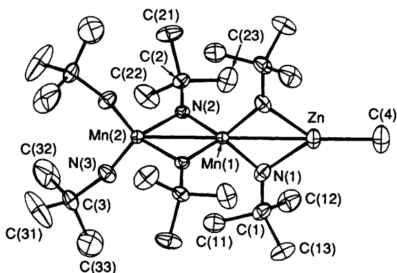
Fig. 6 The structure of the zinc complex 11
