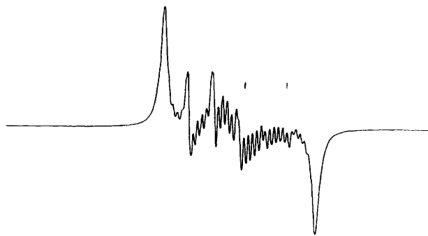
Fig. 5 X-Band EPR spectrum of the mixed-valence Mn^{VI}Mn^V complex Mn_2(NBu)_2(\mu-NBu)_4ZnMe 11 in toluene at 293 K; scale indicates 100 G
