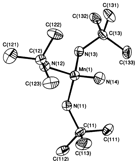
Fig. 1 Structure of [\text{Mn}(\text{N})(\text{NBU})_3]^{2-} in [\text{Li}(\text{OEt}_2)]_2[\text{Mn}(\text{N})(\text{NBU})_3] \cdot \text{LiCl} 2
