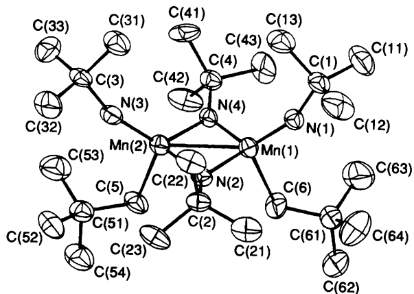
Fig. 3 Structure of [\text{Mn}(\text{CH}_2\text{CMe}_3)(\text{NBu}^t)(\mu\text{-NBu}^t)]_2 7
