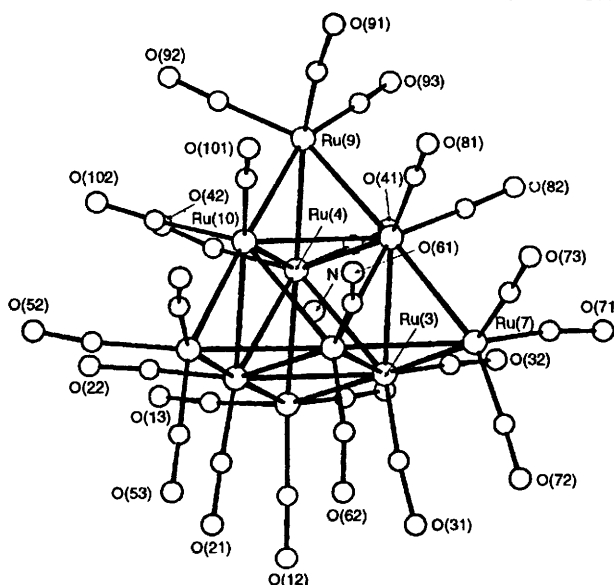
Fig. 3 Structure of [\text{Ru}_{10}\text{N}(\text{CO})_{24}]^{-} 4
