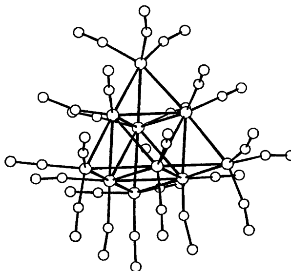
Fig. 2 Structure of [\text{Ru}_{10}\text{C}(\text{CO})_{24}]^{2-} 3
