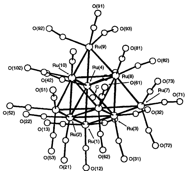
Fig. 1 Structure of [\text{Ru}_{10}\text{H}(\text{C})(\text{CO})_{24}]^{-} 2
