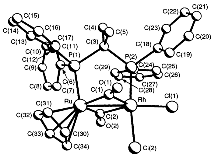
Fig. 3 Molecular structure of [(\eta\text{-C}_5\text{H}_5)\text{Ru}(\mu\text{-CO})_2(\mu\text{-}2,2\text{-dppp})\text{RhCl}_2](\text{Rh-Ru}) 6
