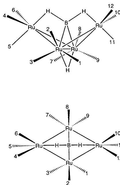
Fig. 1 Numbering scheme for the CO ligands in [\text{Ru}_4\text{H}(\text{CO})_{12}\text{BH}_2] . The lower diagram views the butterfly framework from above and the hinge hydride is under the boron atom
