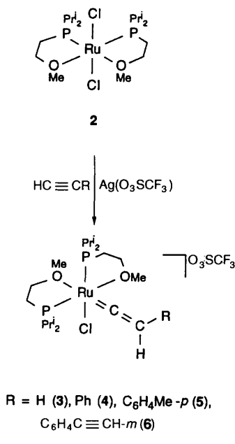
Scheme 2
