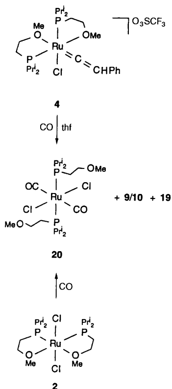
Scheme 6
