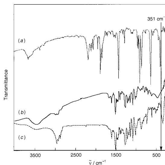
Fig. 2 Infrared spectra of [\text{PPh}_4]_2[\text{Fe}_4\text{S}_4\text{Cl}_4] (a), 2d (b) and 1d (c)
