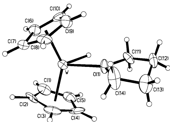
Fig. 1 Molecular structure of the cation of complex 4
