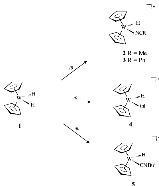
Scheme 1 Synthesis of cationic hydride complexes 2–5 . (i) 1 mol equivalent CF_3SO_3Me , L ( L = MeCN, PhCN or thf ), 0 °C; (ii) 1 mol equivalent CF_3SO_3Me , CNBU^{\dagger} , thf , 0 °C
