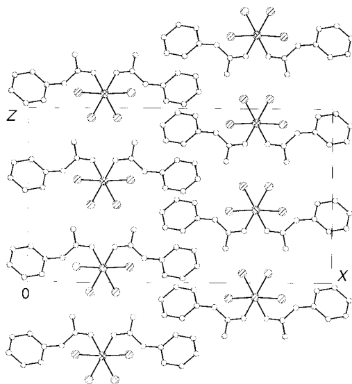
Fig. 4 The ac projection of the unit cell showing the [\text{ReCl}_4(\text{NH}=\text{C}-\text{MeNHPh})_2] molecular dispositions
