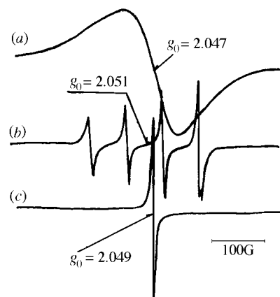
Fig. 4 The ESR spectra of [NEt 4 ] 2 [Cu(C 3 S 4 O) 2 ] 3 in the solid state (a) and in acetonitrile at room temperature (b), together with that of [NEt 4 ] 2 [Ni(C 3 S 4 O) 2 ] in acetonitrile (c). G = 10^{-4} T
