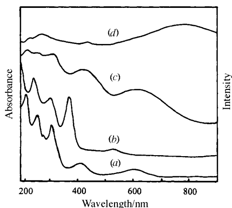
Fig. 3 Electronic absorption spectrum of complex 1 in acetonitrile ( 1.0 \times 10^{-4} mol dm -3 ) [newly resolved (a) and on standing for 1 d in air (b)] and powder reflectance spectra of 1 (c) and 4 (d)
