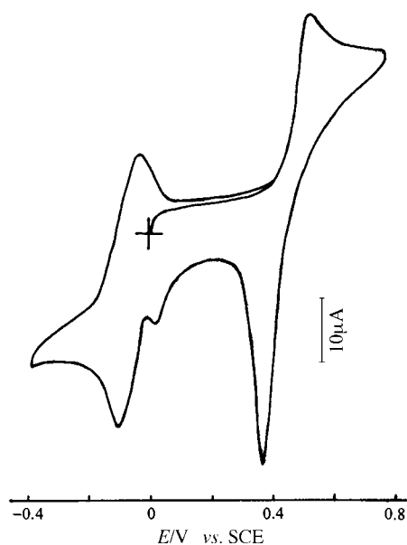
Fig. 5 Cyclic voltammogram of [\text{Ni}(\text{C}_3\text{S}_4\text{O})_2] 1 ( 5 \times 10^{-4} mol \text{dm}^{-3} ) in acetonitrile containing [\text{NBu}_4][\text{ClO}_4] ( 0.1 mol \text{dm}^{-3} ), scan rate 100 \text{mV s}^{-1}
