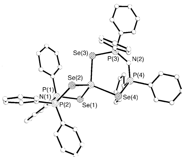
Fig. 3 Molecular structure of [Hg{N(PPh 2 ) 2 -Se,Se'} 2 ] 4 ; the structure complex of 3 is quite similar (hydrogen atoms omitted for clarity)
