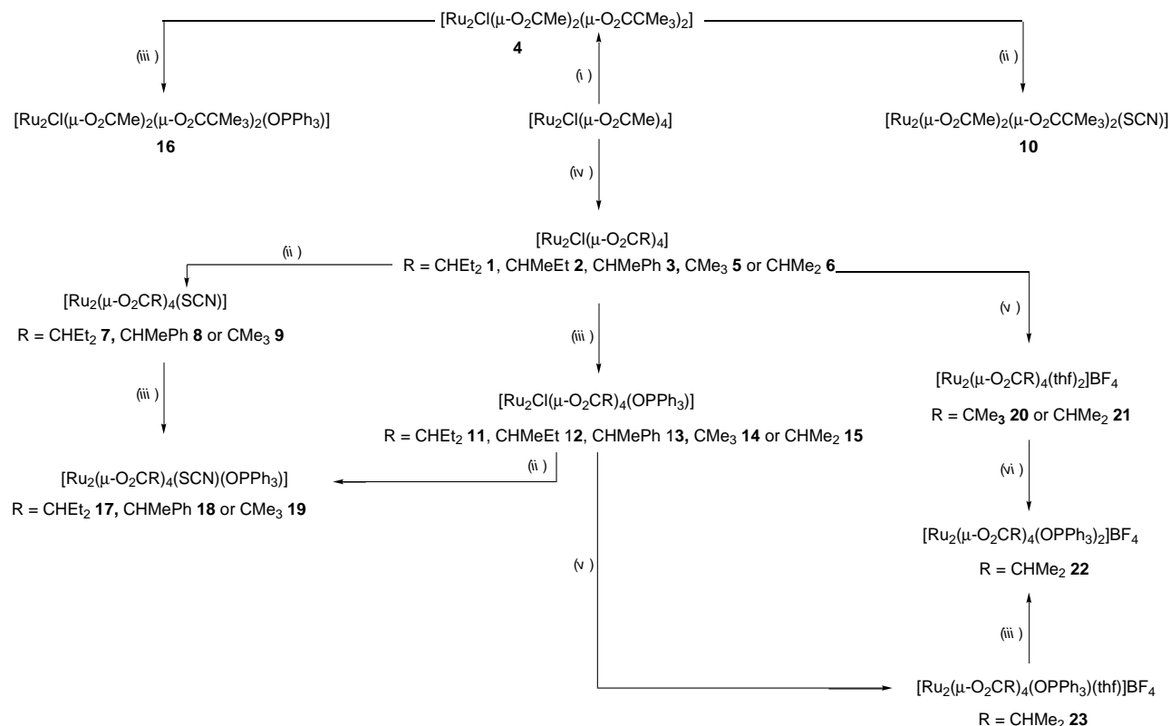
Scheme 1 Synthetic routes to the complexes. (i) 2\text{HO}_2\text{CR} , \text{MeOH} -water; (ii) \text{AgSCN} , \text{thf} ; (iii) \text{OPPh}_3 , acetone; (iv) 6\text{HO}_2\text{CR} , \text{MeOH} -water; (v) \text{AgBF}_4 , \text{thf} ; (vi) 2\text{OPPh}_3 , \text{thf}
