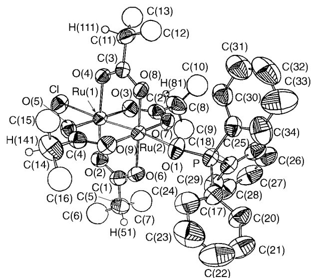
Fig. 1 An ORTEP 22 view of [Ru 2 Cl(μ-O 2 CCHMe 2 ) 4 (OPPh 3 )] showing the atom-numbering scheme. The methyl and phenyl hydrogen atoms are omitted for clarity
