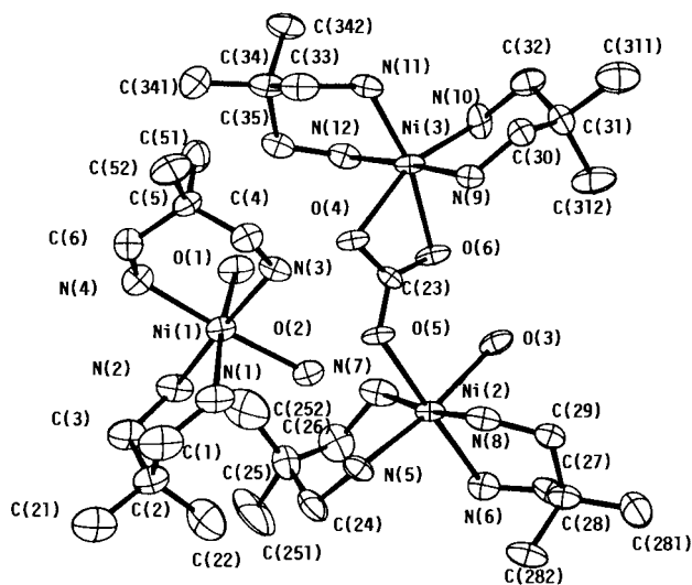
Fig. 1 An ORTEP 15 drawing of [Ni 2 (μ-CO 3 )(dmpd) 4 (H 2 O)][Ni(dmpd) 2 (H 2 O) 2 ][ClO 4 ] 4 ·H 2 O with the atom labelling scheme. Thermal ellipsoids are at the 50% probability level
