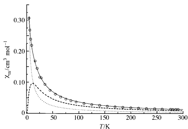
Fig. 3 Plot of \chi_m vs. T for [\text{Ni}_2(\mu\text{-CO}_3)(\text{dmpd})_4(\text{H}_2\text{O})][\text{Ni}(\text{dmpd})_2(\text{H}_2\text{O})_2][\text{ClO}_4]_4 \cdot \text{H}_2\text{O} . The solid line shows the best fit obtained whereas the dashed and dotted lines show the contributions of the dinuclear subunit [\text{Ni}(2), \text{Ni}(3)] and the mononuclear subunit \text{Ni}(1) respectively
