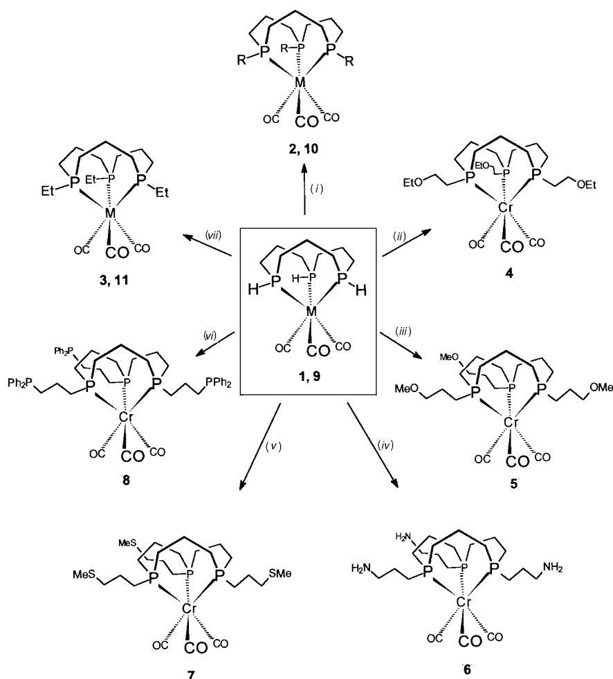
Scheme 1 M = Cr or Mo. (i) (a) 3LiBu, tetrahydrofuran (thf), -78 °C; (b) 3 RX (X = halide), -20 °C, R = Me or PhCH 2 ; (ii) 3EtOC 2 H 5 , azobis(isobutyronitrile) (aibn), 80 °C; (iii) 3MeOC 3 H 5 , aibn, 80 °C; (iv) H 2 NC 3 H 5 , aibn, 80 °C; (v) 3MeSC 3 H 5 , aibn, 80 °C; (vi) Ph 2 PC 3 H 5 , aibn, 80 °C; (vii) 3C 2 H 4 , aibn, 80 °C, 6 atm (ca. 6 × 10 5 Pa)
