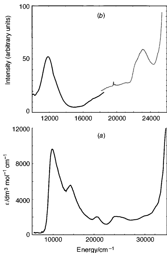
Fig. 6 The UV/VIS spectra of (a) [\text{Co}\{\text{CH}(\text{C}_5\text{H}_4\text{N}-2)_3\}_2]^+ (ethanol solution) and (b) [\text{Co}\{\text{CH}(\text{C}_5\text{H}_4\text{N}-2)_3\}_2]^{2+} at 15 K [KBr disc and single crystal (---)]
