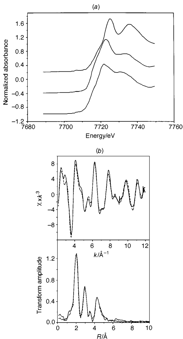
Fig. 5 (a) Normalized cobalt-edge XANES (X-ray absorption near-edge structure) profiles of [Co{P(C 5 H 4 N-2) 3 } 2 ][ClO 4 ] 3 (top), [Co{P(C 5 H 4 N-2) 3 } 2 ][NO 3 ] 2 and [Co{P(C 5 H 4 N-2) 3 } 2 ][ClO 4 ] (bottom). (b) The EXAFS (top) and Fourier transform of [Co{P(C 5 H 4 N-2) 3 } 2 ][ClO 4 ]. —, Experiment; ---, simulation
