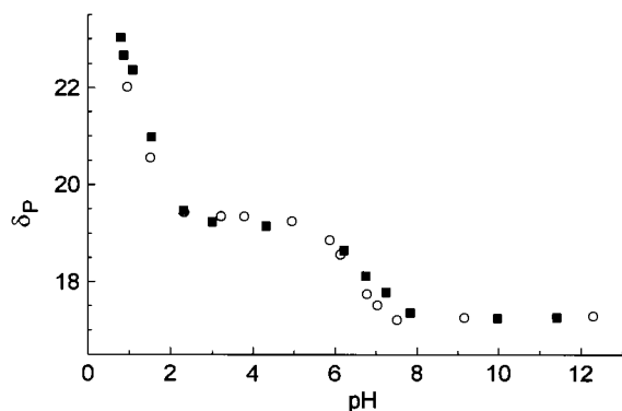
Fig. 7 Plot of \delta_p vs. -\log[\text{H}^+] for the phosphonic group of ( S,S )- (○) and ( S,R )-Met-Ala-( P ) (■)
