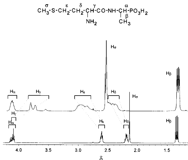
Fig. 9 The ^1\text{H} NMR spectra of free ( S,R )-Met-Ala-( P ) (lower) and a mixture of its complexes with \text{Pd}^{\text{II}} at pD 4.32 ( c_{\text{Pd}} = 0.075 , c_{\text{H,A}} = 0.15 mol \text{dm}^{-3} )
