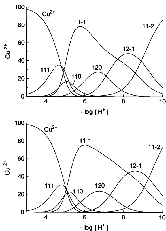
Fig. 2 Distribution diagrams of complexes formed in the \text{Cu}^{2+} -( S,R )-Met-Ala-( P ) (upper) and -( S,S )-Met-Ala-( P ) (lower) systems as a function of -\log[\text{H}^+] ( c_{\text{Cu}} = 0.0025 , c_{\text{H}_2\text{A}} = 0.005 \text{ mol dm}^{-3} )
