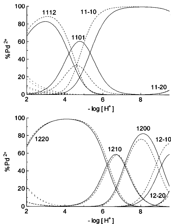
Fig. 5 Distribution diagrams of the complexes formed in Pd 2+ -( S,S )- (full line) and -( S,R )-Met-Ala-( P ) (dashed line) as a function of -\log[H^+] [ c_{Pd} = 0.005 , c_{HA} = 0.005 (upper), 0.01 mol dm -3 (lower)]. Dotted lines (low abundance, region pH 2-4) correspond to [PdCl_{4-n}(H_2O)_n]^{n-2} species.
