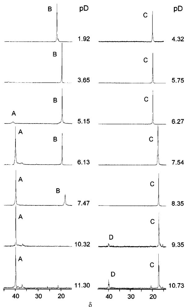
Fig. 8 The ^{31}\text{P} - \{^1\text{H}\} NMR spectra of \text{Pd}^{\text{II}} -Met-Ala-( P ) as a function of pD: left, ( S,R )-Met-Ala-( P ), \text{M}:\text{H}_2\text{A} = 1:1 ( c_{\text{Pd}} = 0.15 , c_{\text{H}_2\text{A}} = 0.15 mol \text{dm}^{-3} ); right, ( S,S )-Met-Ala-( P ), \text{M}:\text{H}_2\text{A} = 1:2 ( c_{\text{Pd}} = 0.075 , c_{\text{H}_2\text{A}} = 0.15 mol \text{dm}^{-3} ). Peaks A belong to dimers 2200 ( 2 \times (1100) ] and their deprotonation and formation of 22–20 [ 2 \times (11-10) ], B to species 1112 and 1102 after deprotonation of the phosphonic group, C to deprotonation of the phosphonic group in 1220 and formation of 1201 and 1200 and consequently deprotonation of the peptide amide group and formation of 12–10 and 12–20 and D probably to a complex of \text{Pd}^{\text{II}} with Ala-( P ) after hydrolysis of the peptide bond
