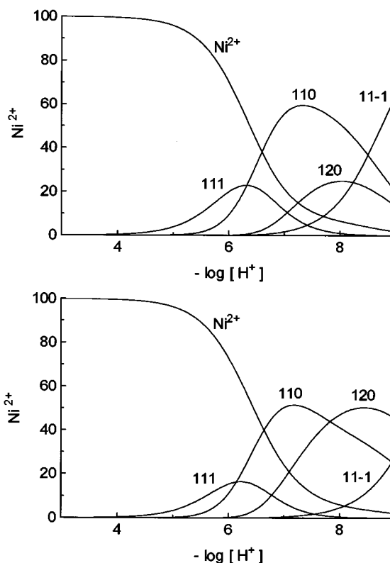
Fig. 3 Distribution diagrams of complexes formed in the \text{Ni}^{2+} -( S,R )-Met-Ala-( P ) (upper) and -( S,S )-Met-Ala-( P ) (lower) systems as a function of -\log[\text{H}^+] ( c_{\text{Ni}} = 0.0025 , c_{\text{H}_2\text{A}} = 0.005 \text{ mol dm}^{-3} )
