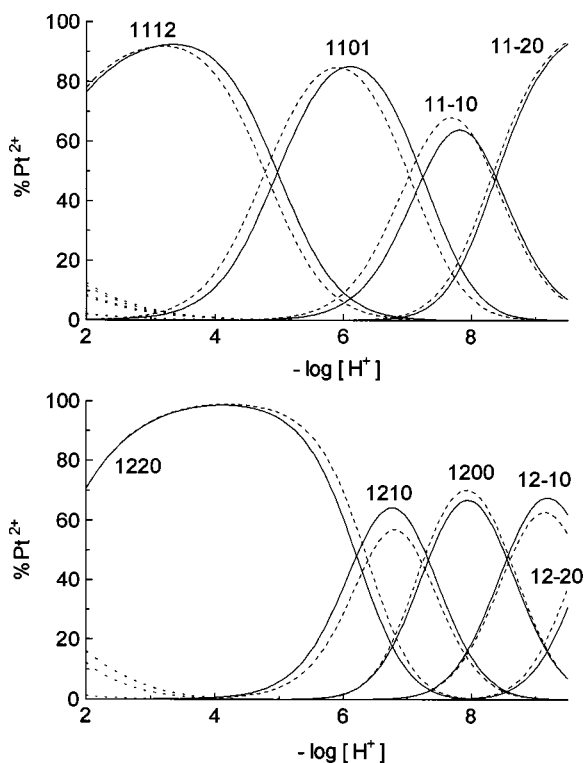
Fig. 4 Distribution diagrams of the complexes formed in Pt 2+ -( S,S )- (full line) and -( S,R )-Met-Ala-( P ) (dashed line) as a function of -\log[H^+] [ c_{Pt} = 0.005 , c_{HA} = 0.005 (upper), 0.01 mol dm -3 (lower)]. Dotted lines (low abundance, region pH 2-4) correspond to [PtCl_{4-n}(H_2O)_n]^{n-2} species.
