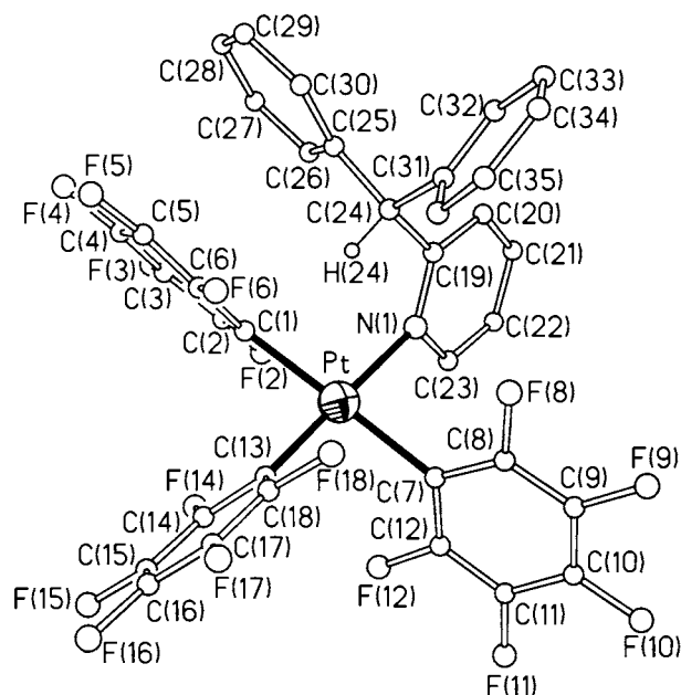
Fig. 1 Crystal structure of the anion of [\text{NBu}_4][\text{Pt}(\text{C}_6\text{F}_5)_3-(\text{NC}_5\text{H}_4\text{CHPh}_2-2)] \cdot 0.5\text{C}_6\text{H}_5\text{Me} , showing the atom labelling scheme. Heavy atoms are represented by their 50% probability ellipsoids
