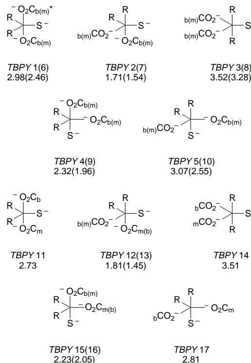
Fig. 3 Calculated quadrupole splitting values for the tin(IV) co-ordination spheres in different stereochemical arrangements with trigonal-bipyramidal ( TBPY ) symmetry of the \text{R}_2\text{S}^{\text{IV}} cation. b = Bidentate, m = monodentate
