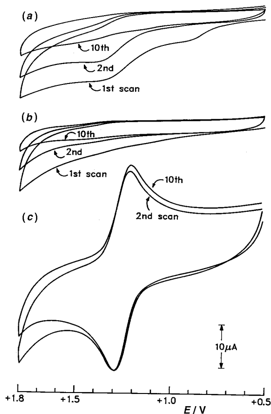
Fig. 3 Cyclic voltammetry between +0.500 and +1.800 V ( 100 \text{ mV s}^{-1} ) of aphen (a), nphen (b), and the complex [\text{Fe}(\text{nphen})_3]^{2+} (c), all present at 1.0 \text{ mol dm}^{-3} in MeCN with 0.10 \text{ mol dm}^{-3} \text{NBu}_4\text{ClO}_4 as electrolyte
