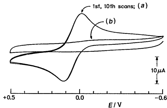
Fig. 4 (a) Electropolymerization of 1.0 \text{ mol dm}^{-3} [\text{Co}(\text{apen})_3]^{2+} on a GCE in MeCN containing 0.10 \text{ mol dm}^{-3} \text{NBu}_4\text{ClO}_4 , cycled 10 times between -0.600 and +0.500 V at a scan rate of 100 \text{ mV s}^{-1} . (b) The electrode from (a) was transferred to a solution containing 0.10 \text{ mol dm}^{-3} \text{NBu}_4\text{ClO}_4 in MeCN and was cycled once over the same potential range using the same scan rate
