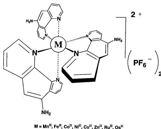
Scheme 1 Structure of the [M(aphen)_3](PF_6)_2 complexes synthesized for electrochemical polymerization
