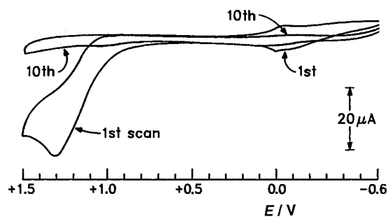
Fig. 5 Electropolymerization of 1.0 mol \text{dm}^{-3} [\text{Cu}(\text{aphen})_3]^{2+} on a GCE in MeCN containing 0.10 mol \text{dm}^{-3} \text{NBu}_4\text{ClO}_4 cycled 10 times between -0.600 and +1.500 V at a scan rate of 100 mV \text{s}^{-1}
