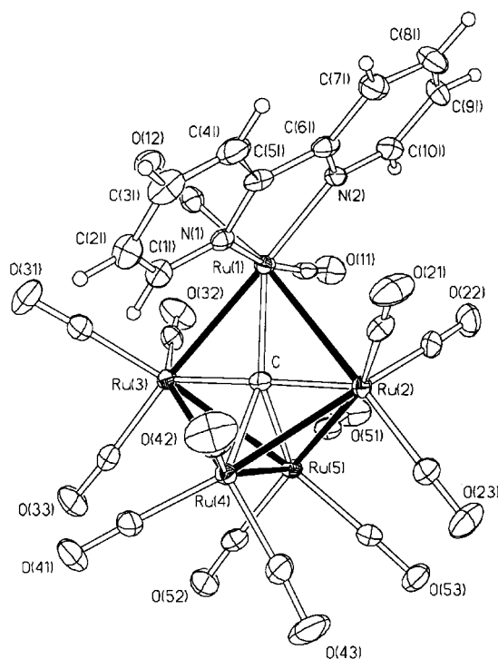
Fig. 1 Thermal ellipsoid plot at 50% probability depicting the molecular structure of [\text{Ru}_5\text{C}(\text{CO})_{14}(\text{bipy})] 3 at 150 K
