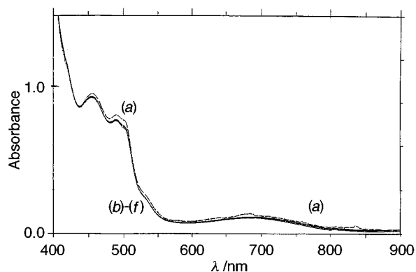
Fig. 3 Spectra of the tpa compound (concentrations of complex and hydrogen peroxide are 10^{-3} and 10^{-1} mol dm ^{-3} , respectively, in acetonitrile, 298 K): (a) 0 min after addition of hydrogen peroxide; (b)–(f) 15, 30, 60, 90 and 150 min after addition
