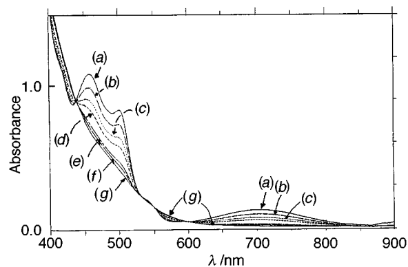
Fig. 4 Spectra of the mep complex (concentrations of iron(III) complex and hydrogen peroxide are 10^{-3} and 10^{-1} mol dm ^{-3} , respectively, in acetonitrile, 298 K): (a) 0 min after addition of hydrogen peroxide; (b)–(g) 15, 30, 60, 90, 150 and 180 min after addition
